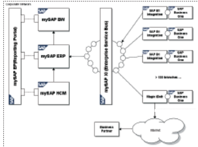
SAP Business One Integration Scenarios
